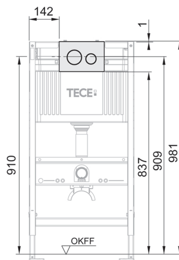
980 mm / 820 mm
